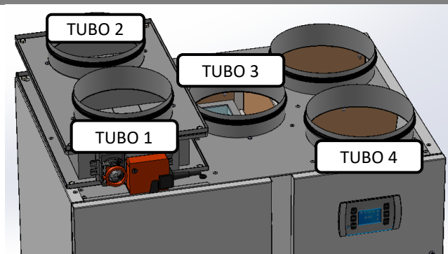
REV 050 VISTA IN ALTO
