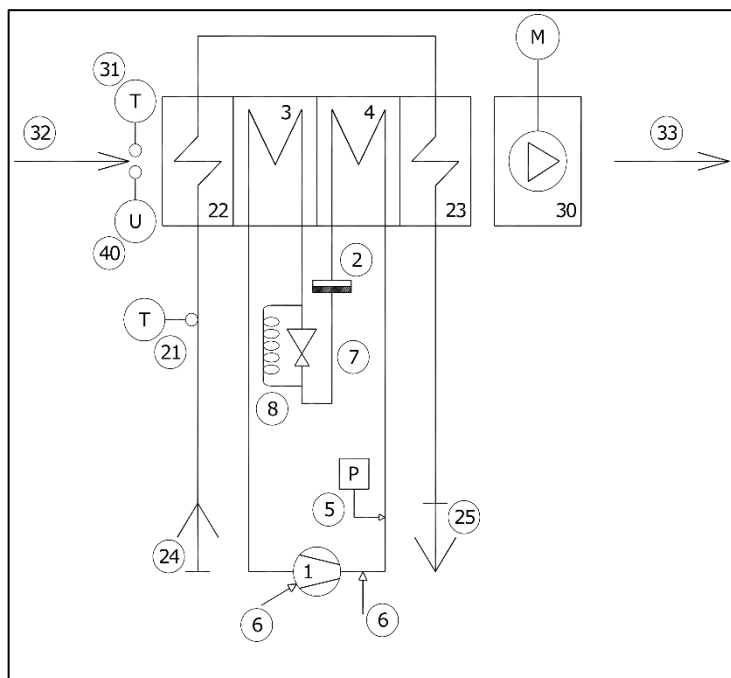
RS_020_035_100_A (isotermico)
